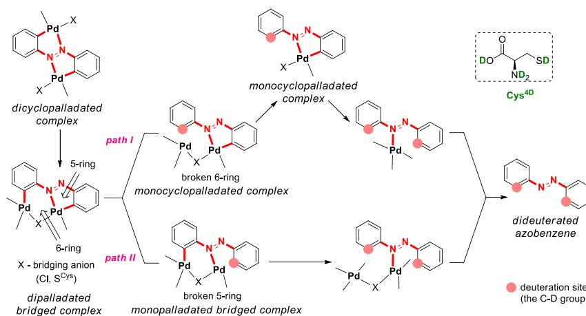
Scheme 1. Deuteration of the palladated azobenzenes.
